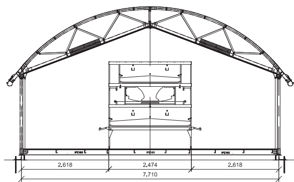
Cross section and top view of the NATURA Camp mobile house with NATURA Step aviary
