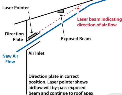
Example 1: Direction plate in correct position
