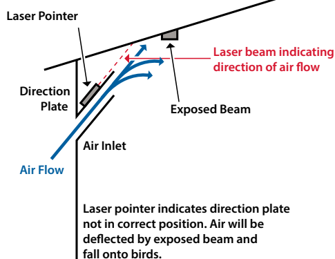
Example 1: Direction plate in wrong position
