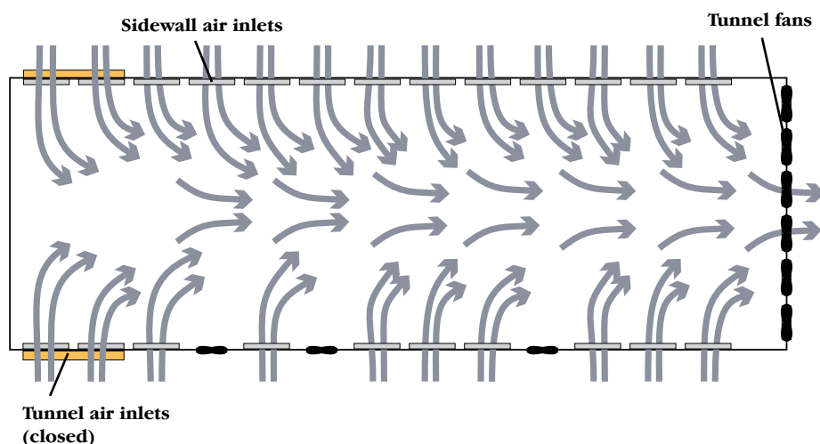
Figure 108: Typical air movement during transitional ventilation.
