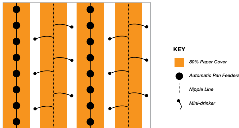
Figure 11: Typical layout of a whole-house brooding system.
