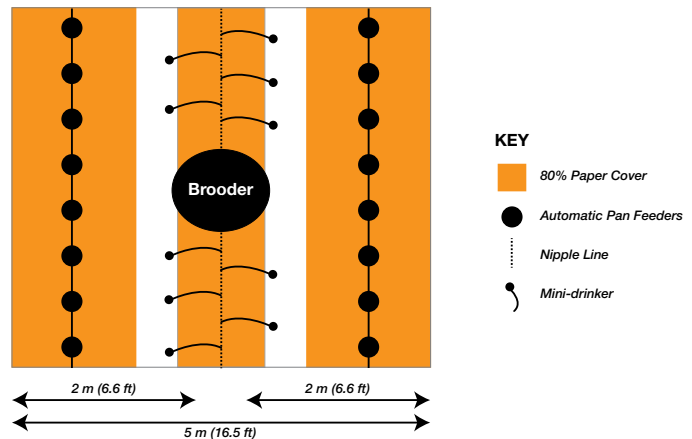
Figure 9: Typical spot brooding layout (1,000 chicks).
