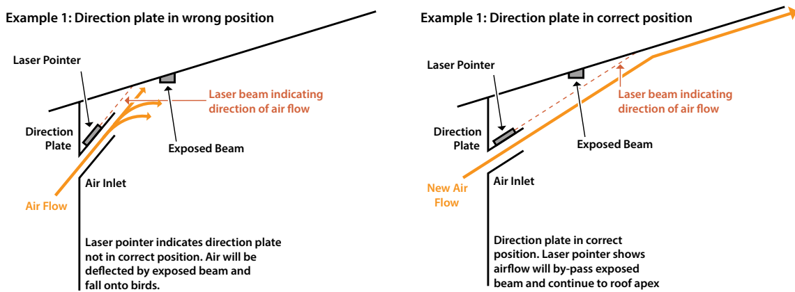
Figure 35: Using a presentation laser to determine if the air direction plate is positioned correctly. A simple laser pointer can be used to provide a visual reference of direction of airflow in to the house. The direction plate can then be set to ensure that airflow bypasses any ceiling obstructions.
